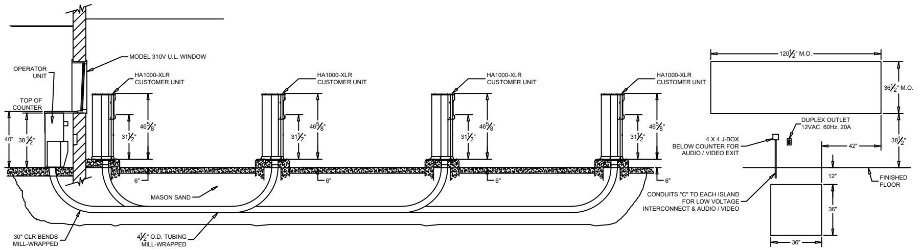
SECTION
